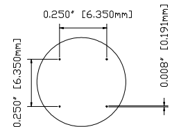
DETAIL A - DOT SPEC SCALE 5:1
